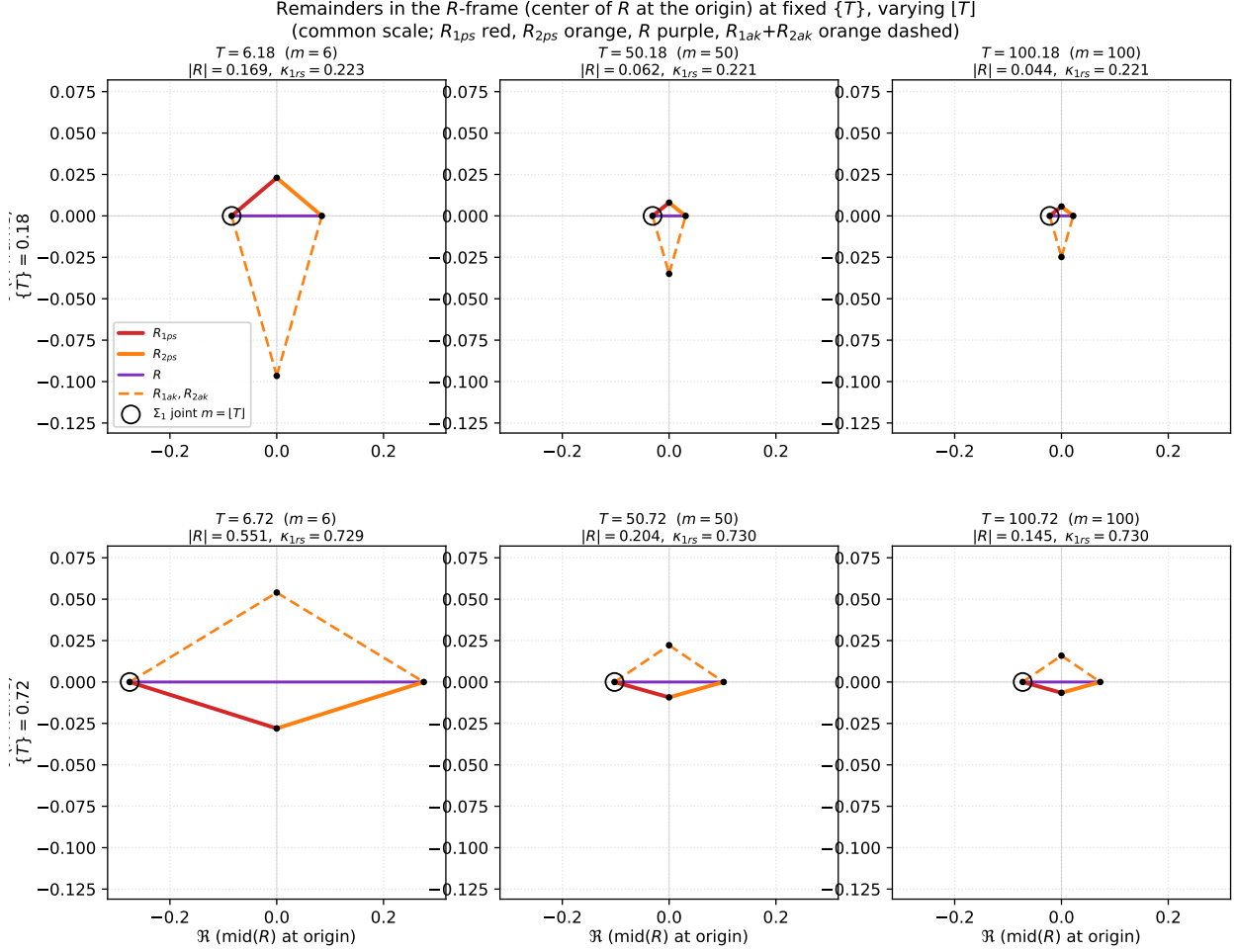
Figure 6: Remainders in the R -frame at fixed fractional part \{T\} , varying [T] . The frame is centered on the midpoint of R (so R runs from -|R|/2 to +|R|/2 on the real axis). Top row: \{T\} = 0.18 at T = 6.18, 50.18, 100.18 . Bottom row: \{T\} = 0.72 at T = 6.72, 50.72, 100.72 . Colors match Figure 5: R_{1ps} red, R_{2ps} orange, R purple, R_{1ak} and R_{2ak} orange dashed. The large open circle marks the left endpoint of R , which is the anchoring joint \Sigma_1 at m = [T] that all three splits leave from. All six panels share the same axis scale. Generated by fig_remainder_scale_panels.py .
