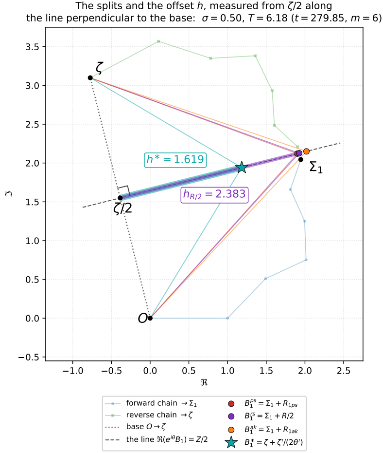
Figure 37: The offset h of (133), drawn at T = 6.18 . Because \Re(e^{i\theta} B_1) = Z/2 for every split, all of the split points lie on one line when \sigma = \frac{1}{2} , the dashed line through \zeta/2 perpendicular to the base O \rightarrow \zeta (the right angle is marked). What distinguishes one split from another is h , the signed distance from \zeta/2 along that line, drawn as a thick stretch of the line for the R/2 split (purple, h_{R/2} = 2.383 ) and for the velocity split (teal, h^* = 1.619 ); the two legs of each split are drawn thin in its own colour and the two chains fainter still. Generated by fig_splits_h.py .
