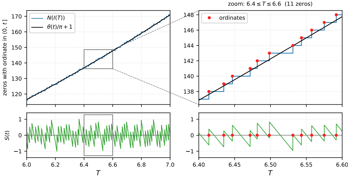
Figure 35: Left : the staircase N(I(T)) (blue) over 6 \leq T \leq 7 , which is 264.9 \leq t \leq 352.9 and carries the 55 ordinates \gamma_{117} through \gamma_{171} , against the smooth part \theta(t)/\pi + 1 of (129) (black). The vertical gap between them is S , which here stays within [-1.002, +1.001] . Right : the boxed window 6.4 \leq T \leq 6.6 magnified, with the eleven ordinates it holds, \gamma_{138} through \gamma_{148} , marked in red at the top of each riser and placed at T = I^{-1}(\gamma) . The risers are unevenly spaced while the smooth part climbs steadily. Below each panel is the gap itself, S (green), which at this magnification shows plainly as a sawtooth: a unit jump at every ordinate and a steady slide between them. Generated by fig_staircase_67.py .
